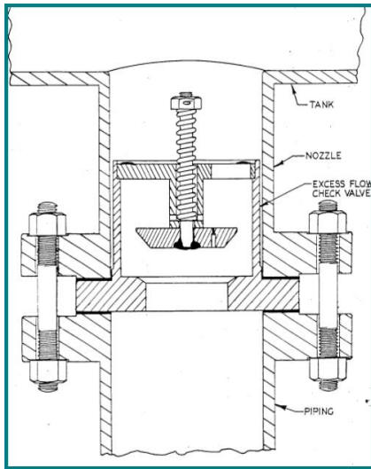
Figure 1: Installation Schematic
